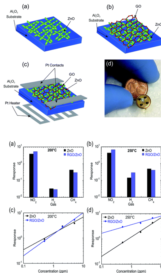
Figure 14: The schematic representation of gas sensor device fabrication. Ref. [167] open access
