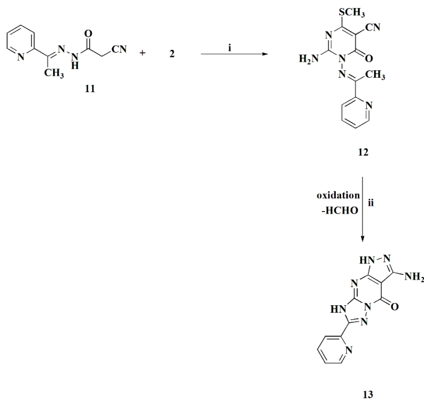
Scheme 3: Synthesis of Pyrazolopyrimidines as bio-isostere purine analogs
