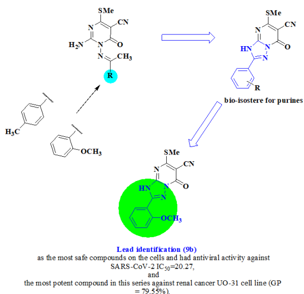
Fig.5. SAR of compound 9b .
