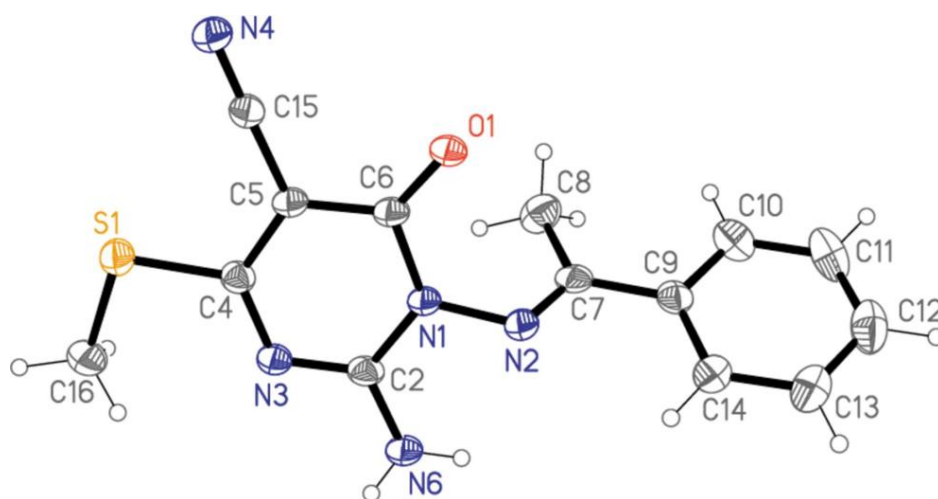
Figure 2: The structure of compound 5a in the crystal. Ellipsoids correspond to levels of 50% probability. “Reproduced with permission of the International Union of Crystallography under the open-access licence” 38
