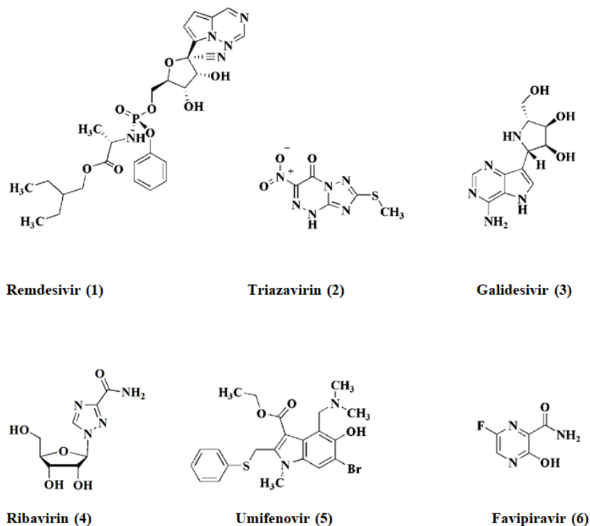
Figure 1: Candidate drugs against SARS-CoV-2 and COVID-19
