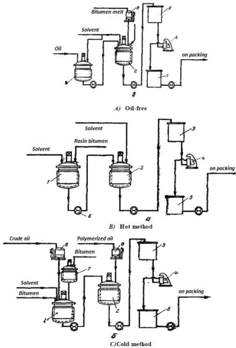
Fig. 2. The scheme of production of bituminous varnishes: 1 - reactor; 2 - mixer; 3 - pressure tank; 4 - super-centrifuge; 5 - receiving tank; 6 - pump; 7 - melter; 8 gauges on scales; 9 - polymerizer.
