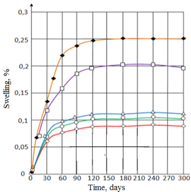
Fig. 3. Swelling of bituminous coatings in water at 25 °C
